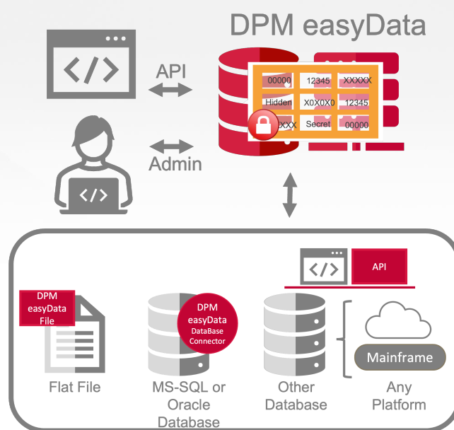
Figure 6 easyData API and no-code database connector
